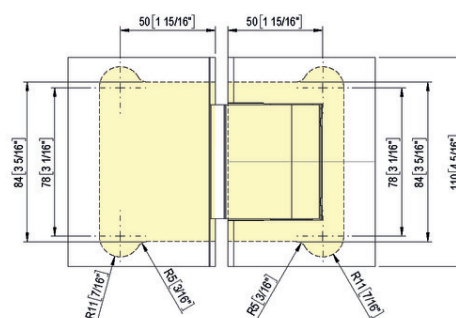
front view 1
